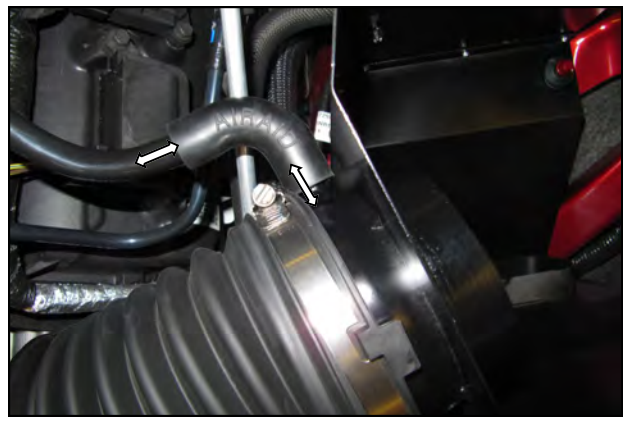
15. On V6 motors, connect the factory crankcase breather hard line to the Airaid Intake Tube using the 90 deg. Breather Elbow (#7). Disregard the 13" Breather Hose (#6) it will not be used.
