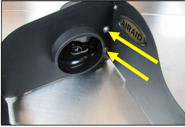
10. Mount the Sensor Tube onto the Panel Assembly and secure using the two 1/4-20 Button Head Screws and 1/4" Flat Washers.
