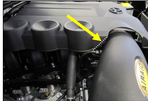
13. Place the engine cover back on top of the motor and note the location where it comes in contact with the Airaid Intake Tube. Remove the cover and trim the edge approximately 1/8" and reinstall.
