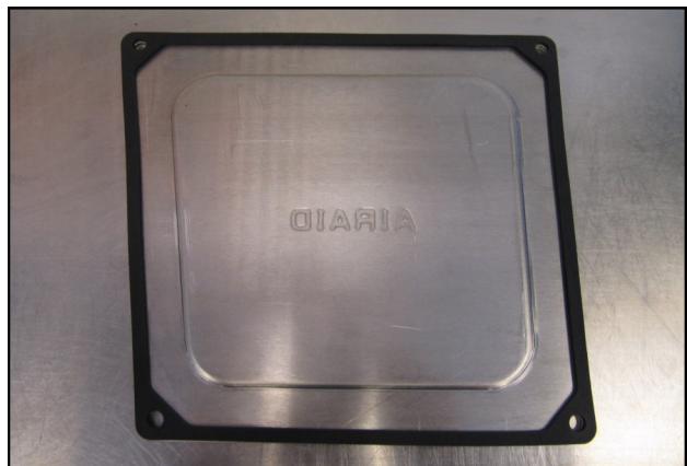
15. Place the Gasket (#8) onto the underside of the Air Box Lid (#4) and peel off the protective film. Mount the lid on the Air Box using four 1/4-20 x 1/2" Button Head Bolts (#16), and 1/4" Flat washers (#17).
