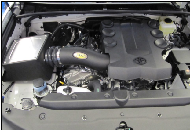
16. Double check your work! Make sure there is no foreign material in the intake path. Make sure all clamps, hoses, bolts, and screws are tight. Double check the hood clearance!
