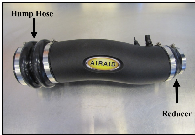
10. Slide the Hump Hose (#6), and two #68 Hose Clamps (#21), onto the Intake Tube as shown. Slide the Reducing Coupler (#7) and the #48 (#19) and #64 Clamps (#20) on the other end of the Intake Tube. Leave the Clamps loose for now.
