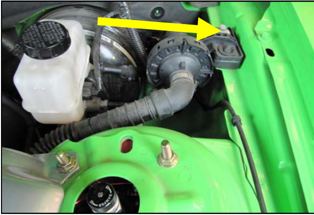
13. Remove the entire Resonator tube assembly and all associated stand offs from the intake tube and the vehicle. Remove the 6mm bolt securing the diaphragm housing to the inner fender remove the tubing from the Fire wall.
