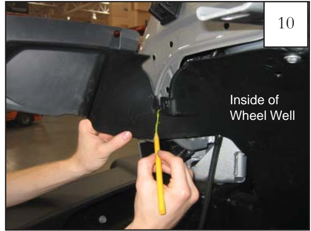
Mark the front portion of the splash shield with a grease pencil in location shown in preparation for trimming. The splash shield should be flush with the sheet metal after being trimmed. NOTE: If trimmed too little, flare won't fit; if trimmed to much, shield won't stay behind flare.
