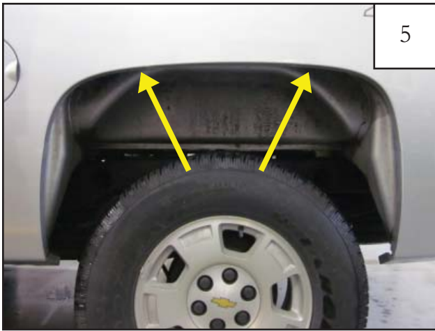
Clip (CL1-0022) locations.
