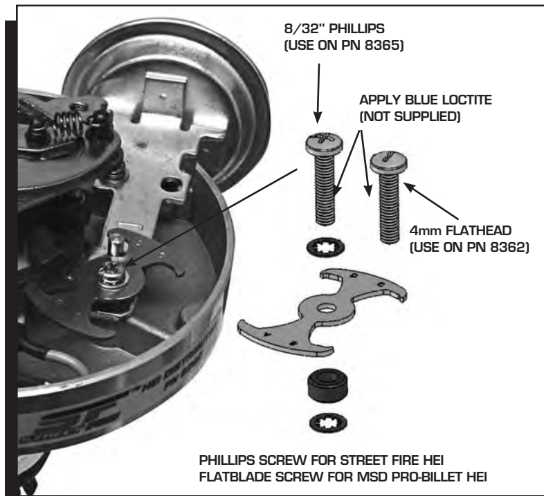
Figure 2 Installation.
