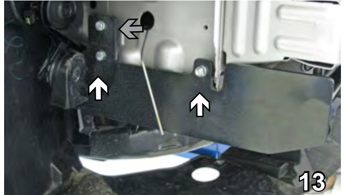
13. On the passenger side, insert 3/8"-16 x 2" hex bolts in all holes, 1" spacers are placed between the baseplate and the frame for each hole. The front hole and the bottom back hole have 3/8" lock washers with 3/8-16 hex nuts (white arrows). The top back hole has the 3/8" lock washer on this side and a 3/8"-16 nut plate inserted into the drilled hole (gray arrow). Be sure to use Loctite Red on all the bolts.
