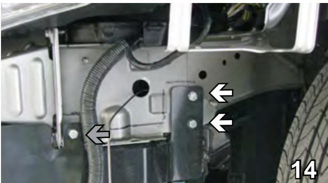
14. On the driver side, insert 3/8"-16 x 2" hex bolt in the front hole (gray arrow), a 1" spacer is placed between the baseplate and the frame, 3/8" lock washer with 3/8"-16 hex nut. The back holes (white arrows) have 3/8-16 x 1-1/2" hex bolts. The bottom back hole has 3/8" lock washer with 3/8"-16 hex nut. The top back hole has the 3/8" lock washer on this side and a 3/8"-16 nut plate inserted into the drilled hole. Be sure to use Loctite Red on all the bolts.
