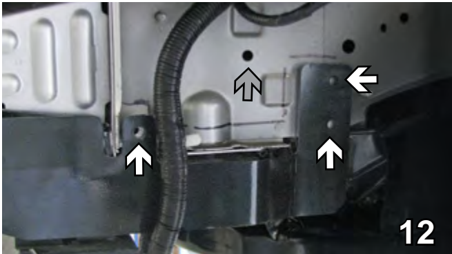
12. Be sure the baseplate is level with respect to the vehicle frame. Using the baseplate as a template with the 13/32" drill bit, drill three (3) holes on the side (white arrows) (make sure baseplate bracket does not bend). Using the 1-1/4" hole saw, drill a hole so that nut plates may be inserted into the frame (gray arrow). Do this to both sides of the vehicle.
