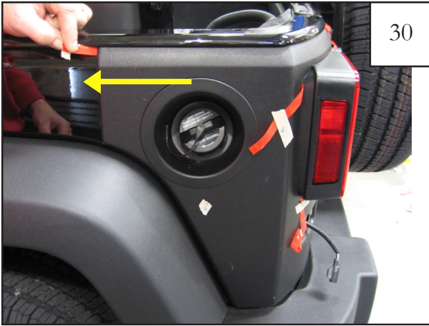
Pull tape liner 5 left toward the front of the vehicle. Press side of part firmly for proper tape adhesion. NOTE: Refer to step 24 for tape liner tab numbering.
