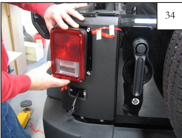
Using a #2 Phillips screwdriver, remove the tail light.
