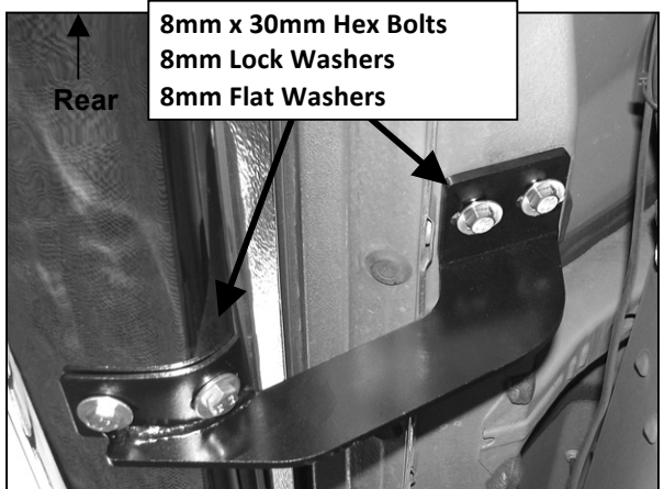
(Fig 5) Driver/Left Rear Bracket Pictured
