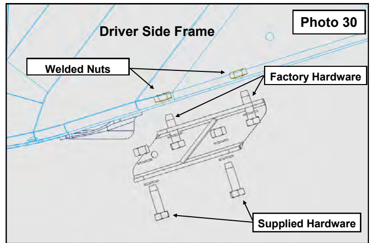
Install swaybar drop bracket and swaybar.
