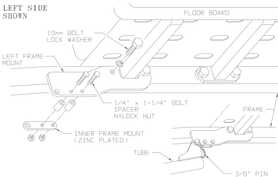
FIGURE 2: FRAME MOUNT INSTALLATION
